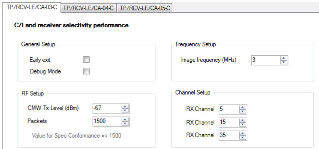
Fig. 3-21: Configuration: Low Energy C/I performance (TP/RCV-LE/CA-03-C)
