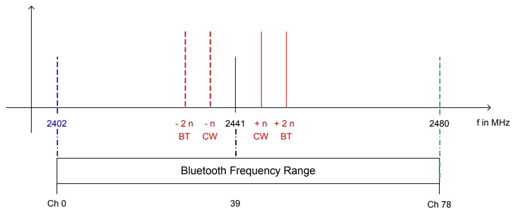
Fig. 3-12: Intermodulation performance
